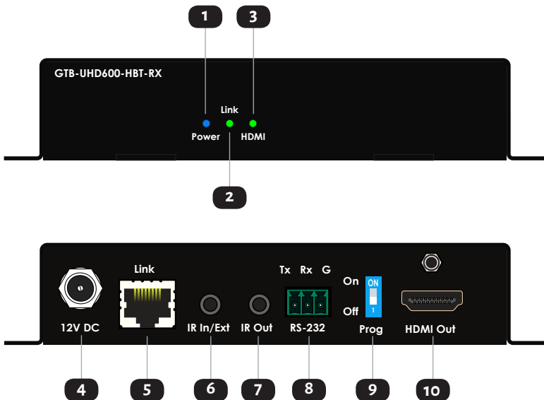
Receiver Unit
